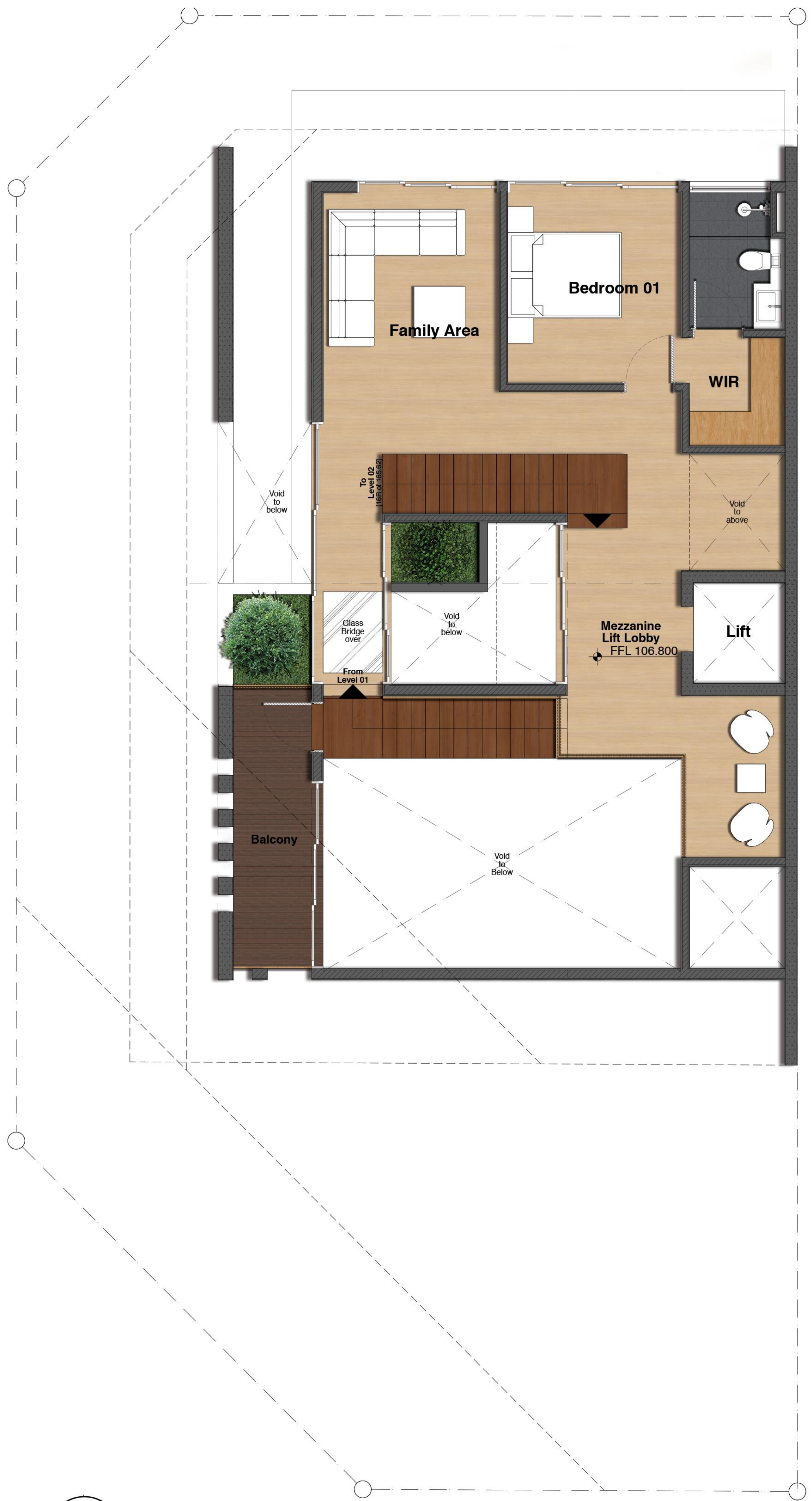
MEZZANINE STOREY PLAN
